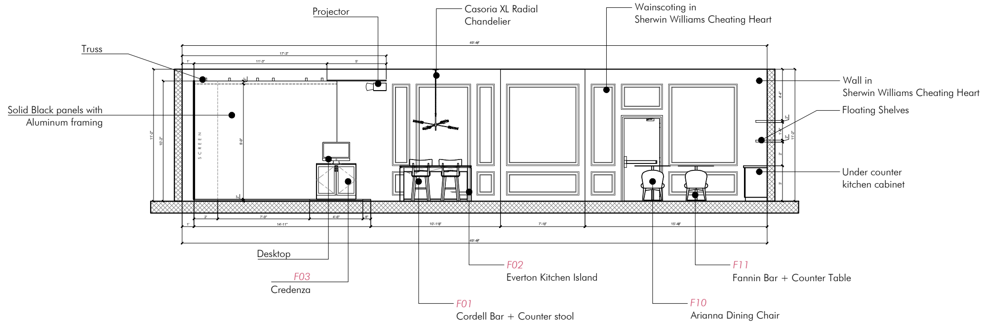
1 SWINGSHAFT SECTIONAL ELEVATION C SCALE : 1/8" = 1'-0"
